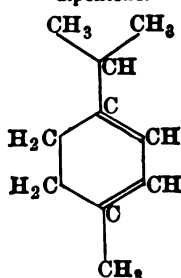
\alpha -Terpinene
